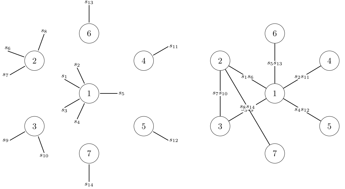
(a) Stubs generated from a scale-free degree sequence (b) Stubs paired into a simple realized graph
